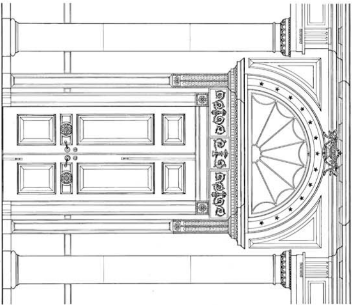
INTERIOR ELEVATION
