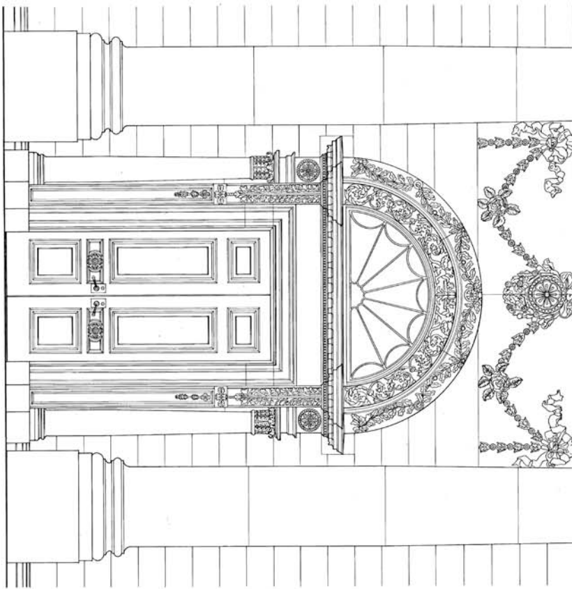
EXTERIOR ELEVATION
