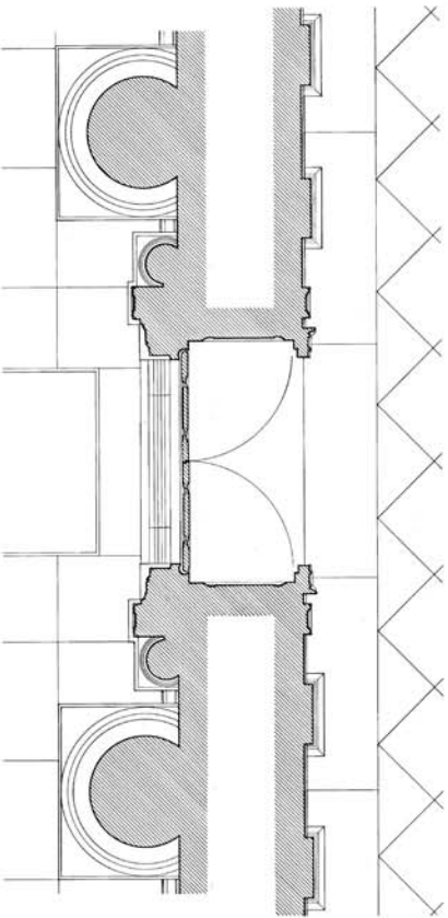
PLAN
